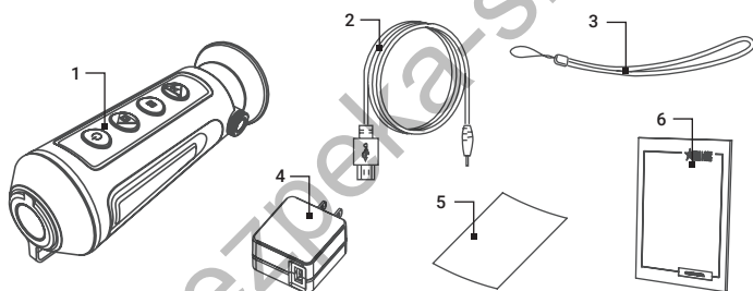
FIGURE 1-2. STANDARD COMPONENTS
